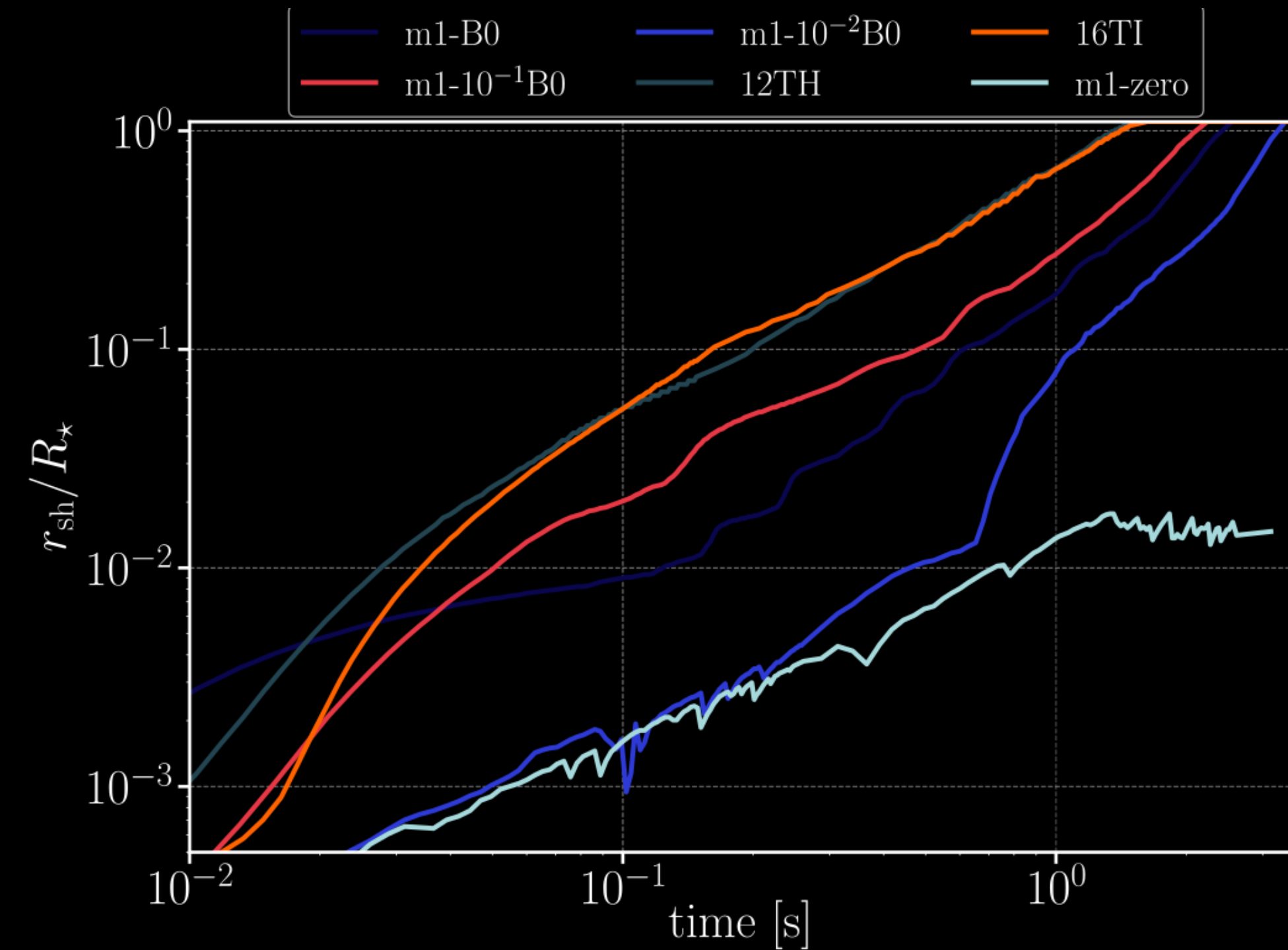
Shock front
